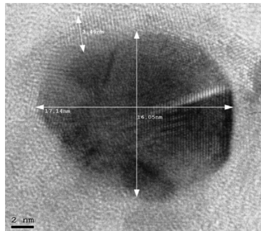
Fig. 8 HRTEM of sample (4) of Au/CdS
