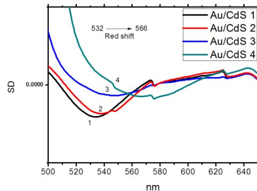
Fig. 7 Second derivative for Au-core region of Au/CdS nanoparticles
